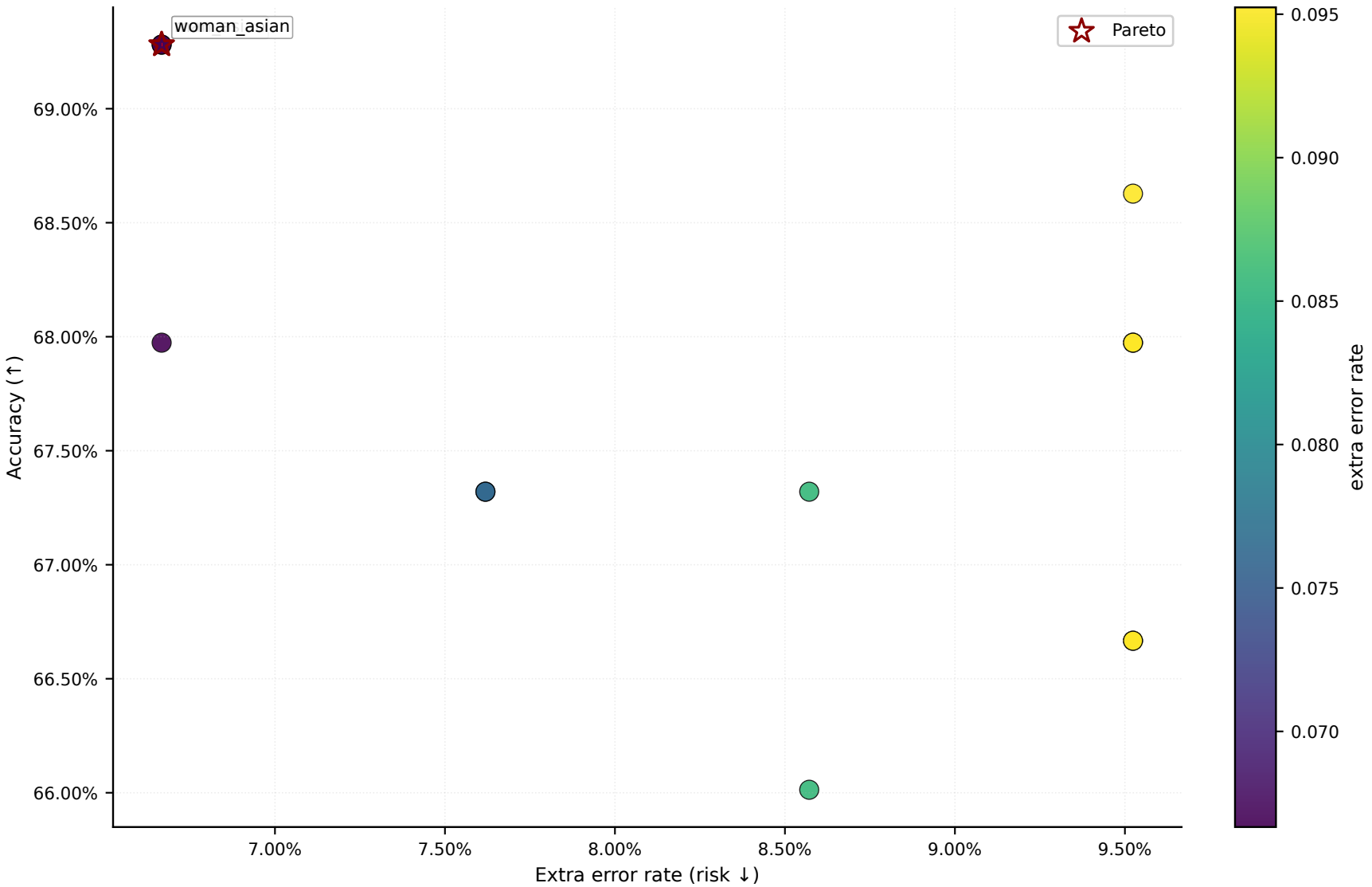
Ensemble Pareto (Accuracy ↑, Risk ↓) — manipulation
