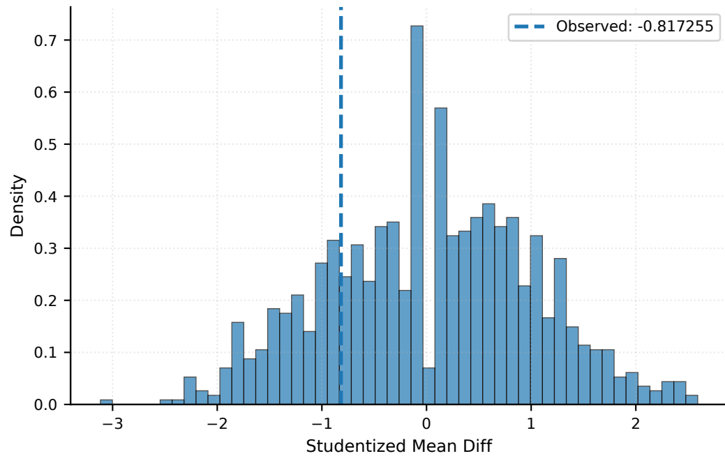
Overall Profile Variance Test p = 0.7093
