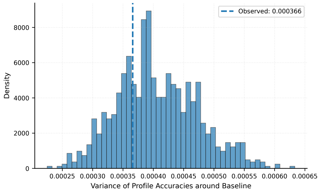
Overall Profile Variance Test p = 0.7093
