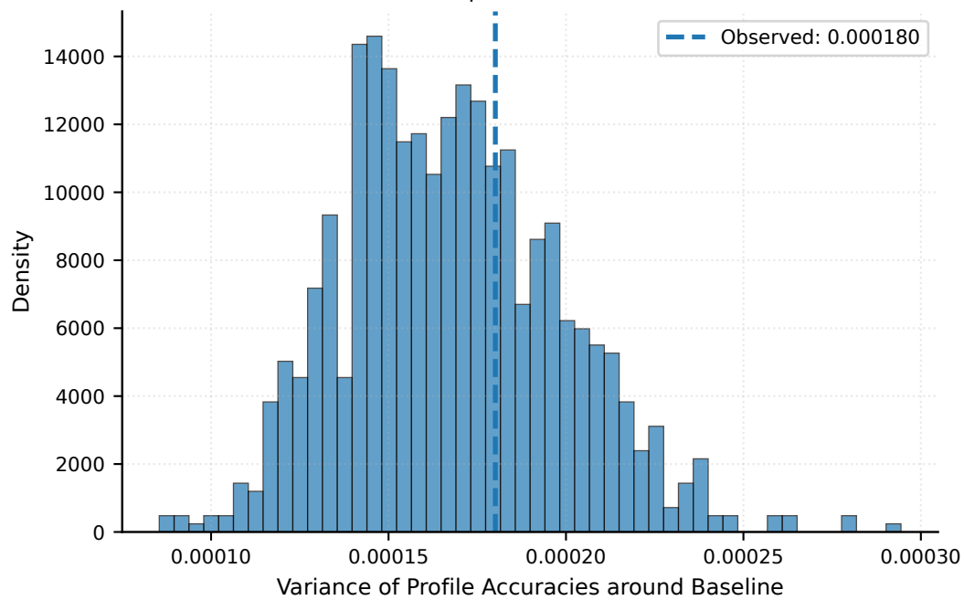
Overall Profile Variance Test p = 0.3327
