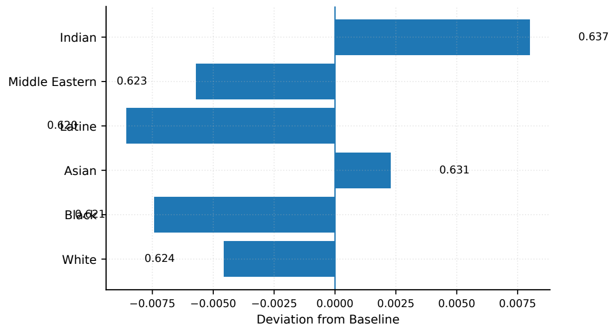
Ethnicity Group Deviations (Baseline: 0.6286)
