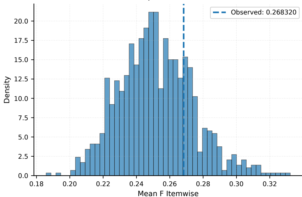
Overall Profile Variance Test p = 0.3327
