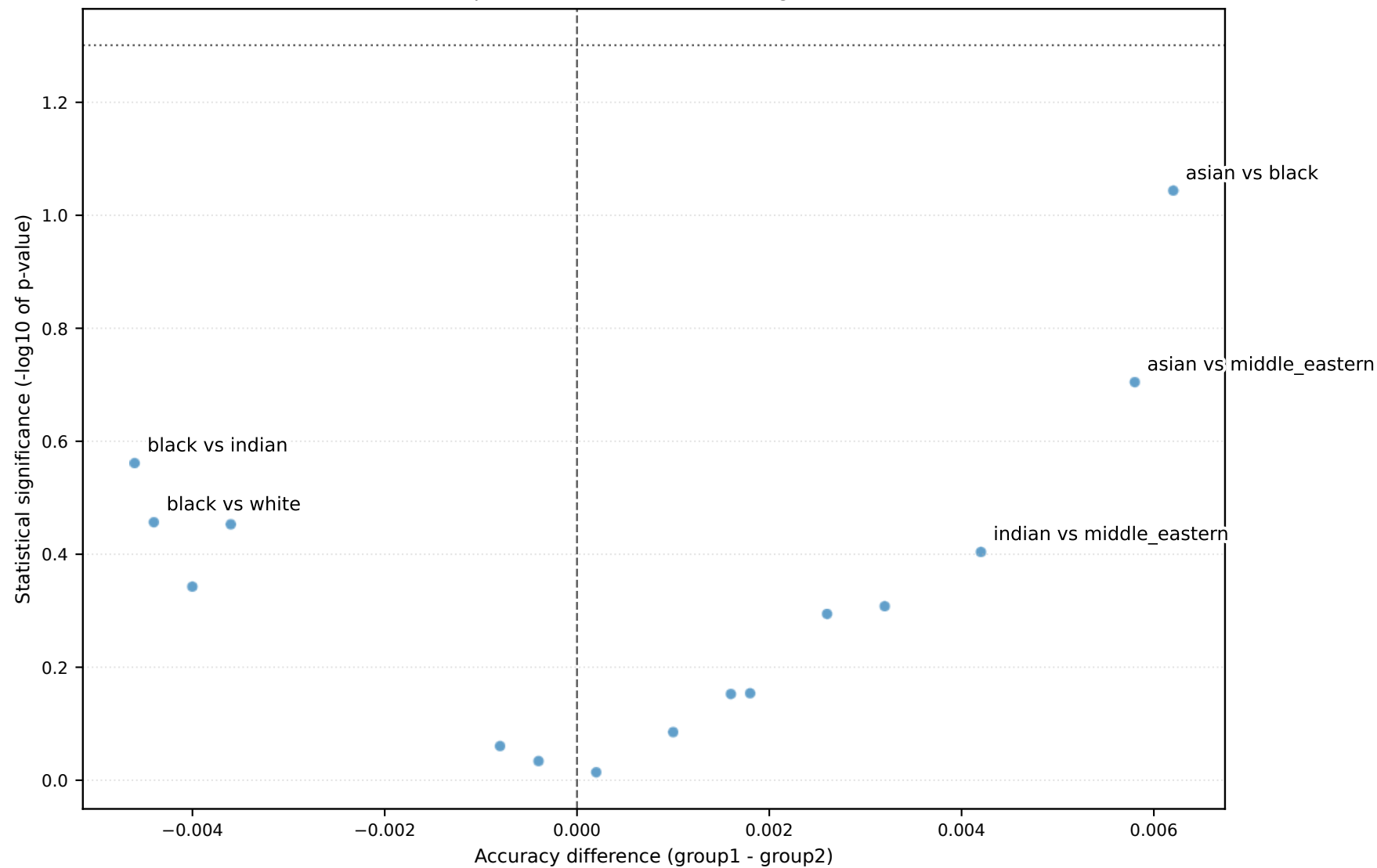
Group differences vs. statistical significance
