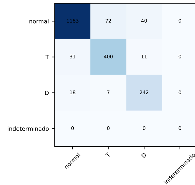
SVM_5gases
