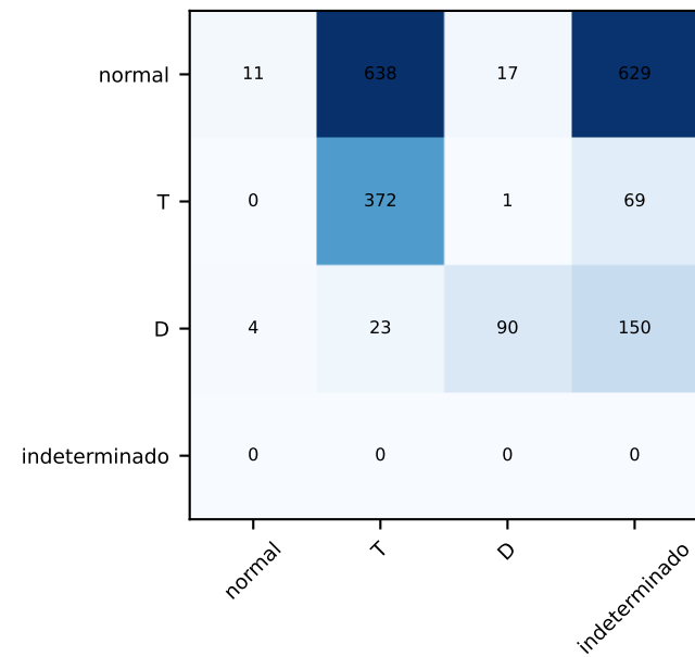
LR
