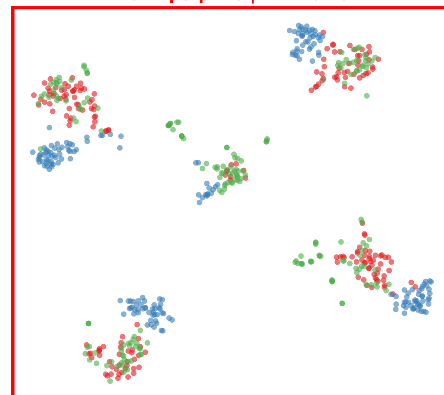
UMAP n=15,md=0.0 | kNN=0.75
