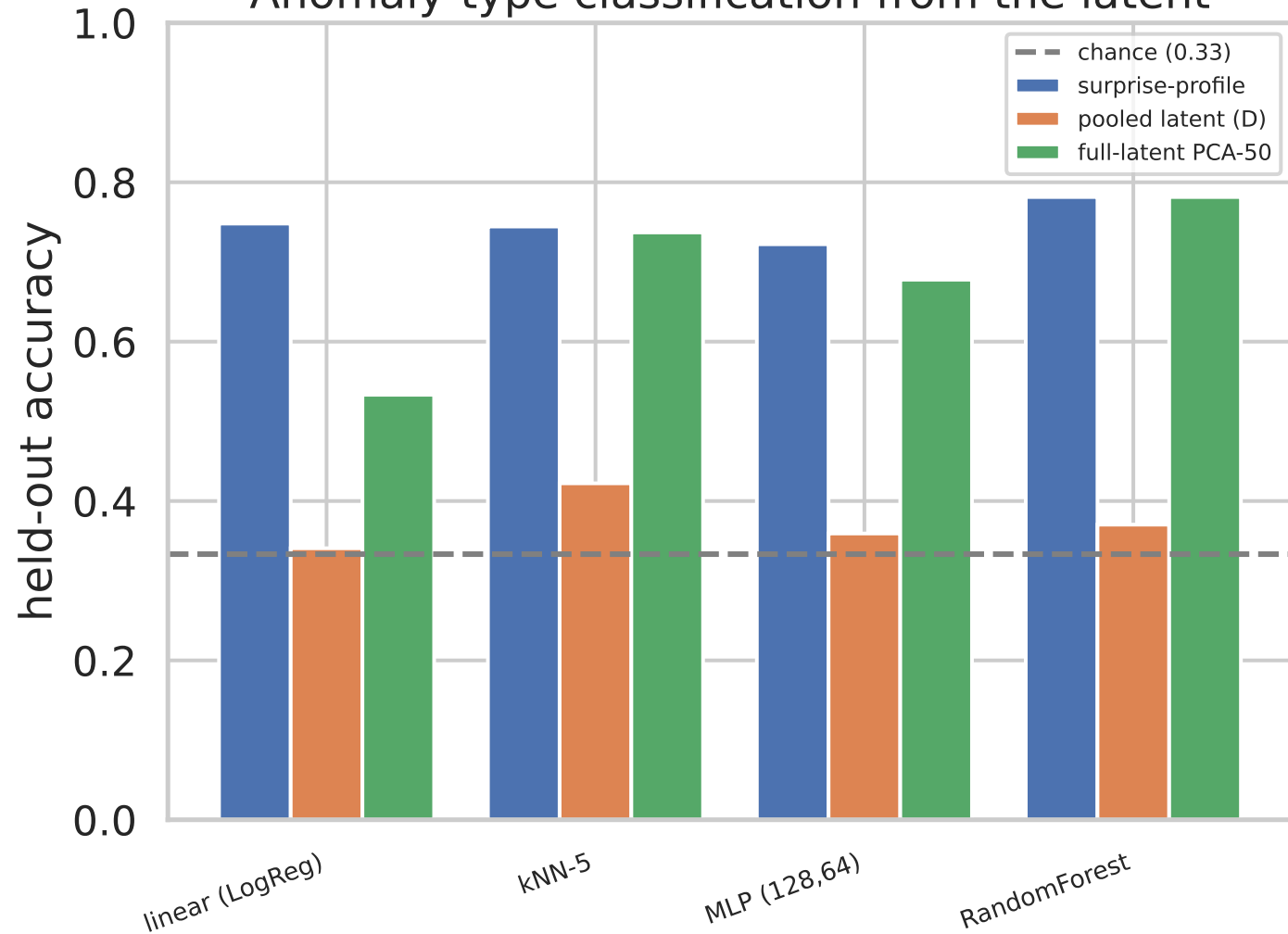
Anomaly-type classification from the latent
