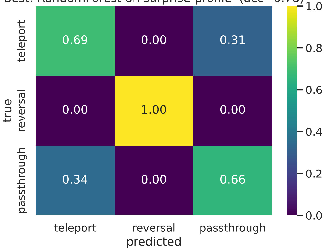
Best: RandomForest on surprise-profile (acc=0.78)
