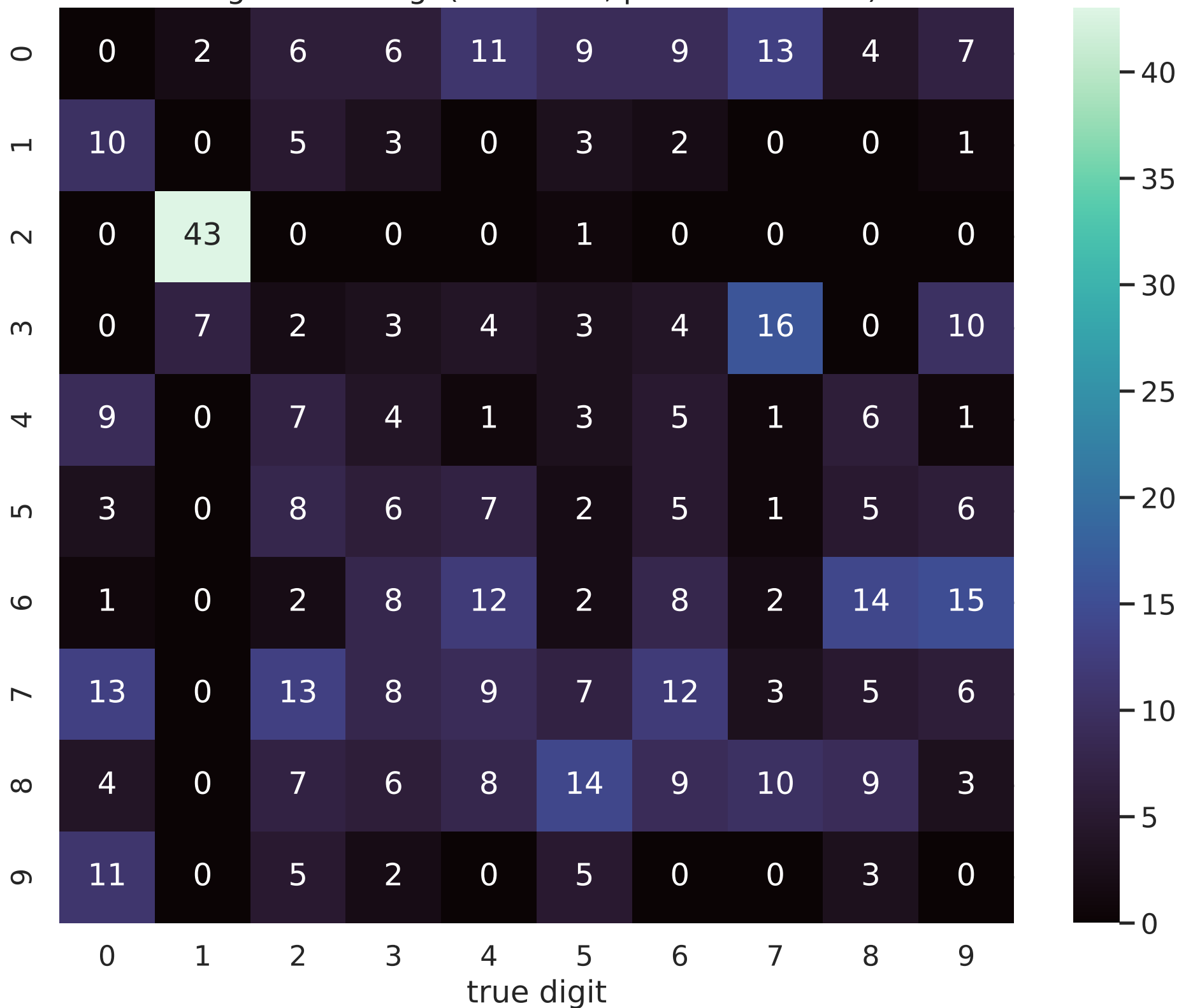
Digit clustering (ARI=0.11, probe acc=0.48)
