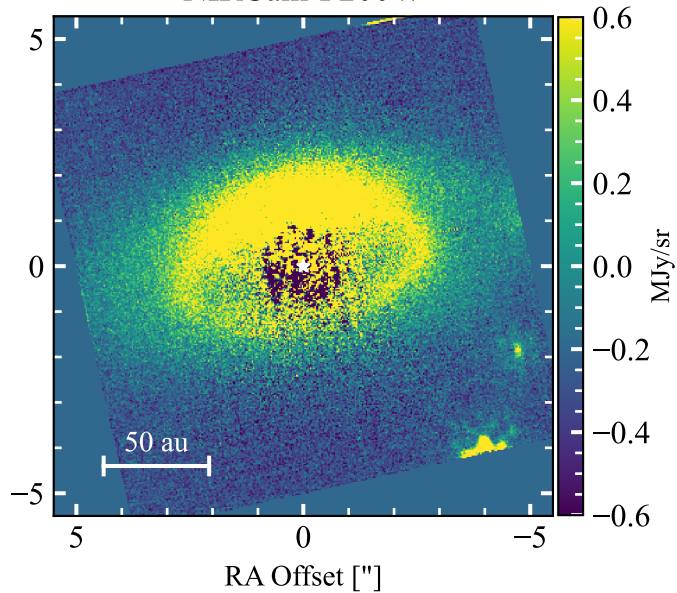
NIRCam-F200W
