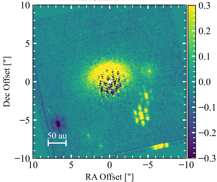
NIRCam-F444W
