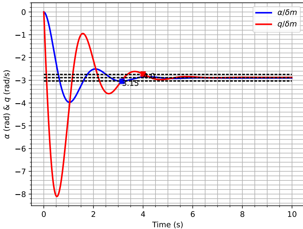
Step response \alpha/\delta m and q/\delta m
