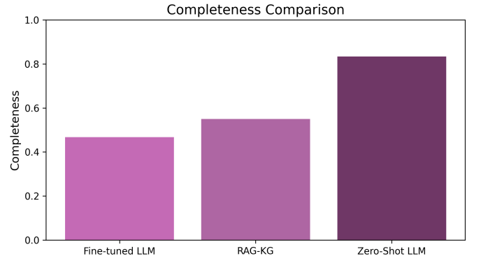
Fig. 20. Completeness on three comparison models.
