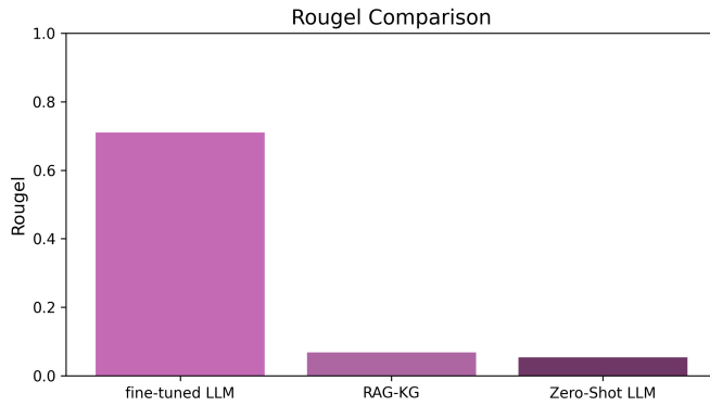
Fig. 13. ROUGE L scores on three comparison models.
