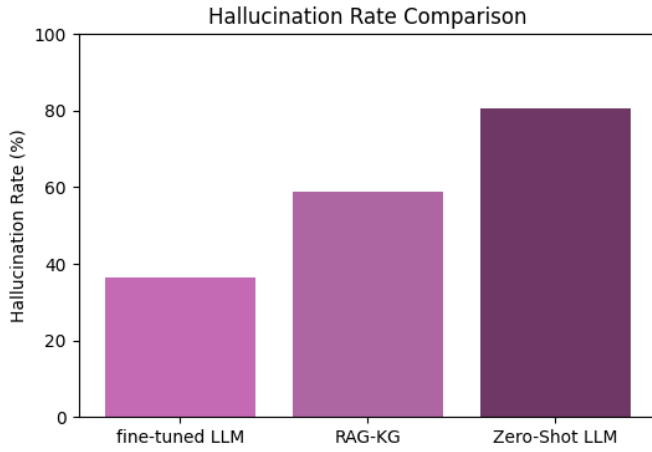
Fig. 22. Hallucination rate % on three comparison models.
