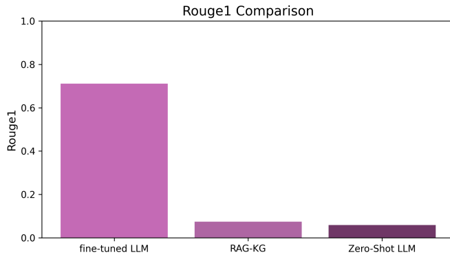
Fig. 11. ROUGE1 scores on three comparison models.
