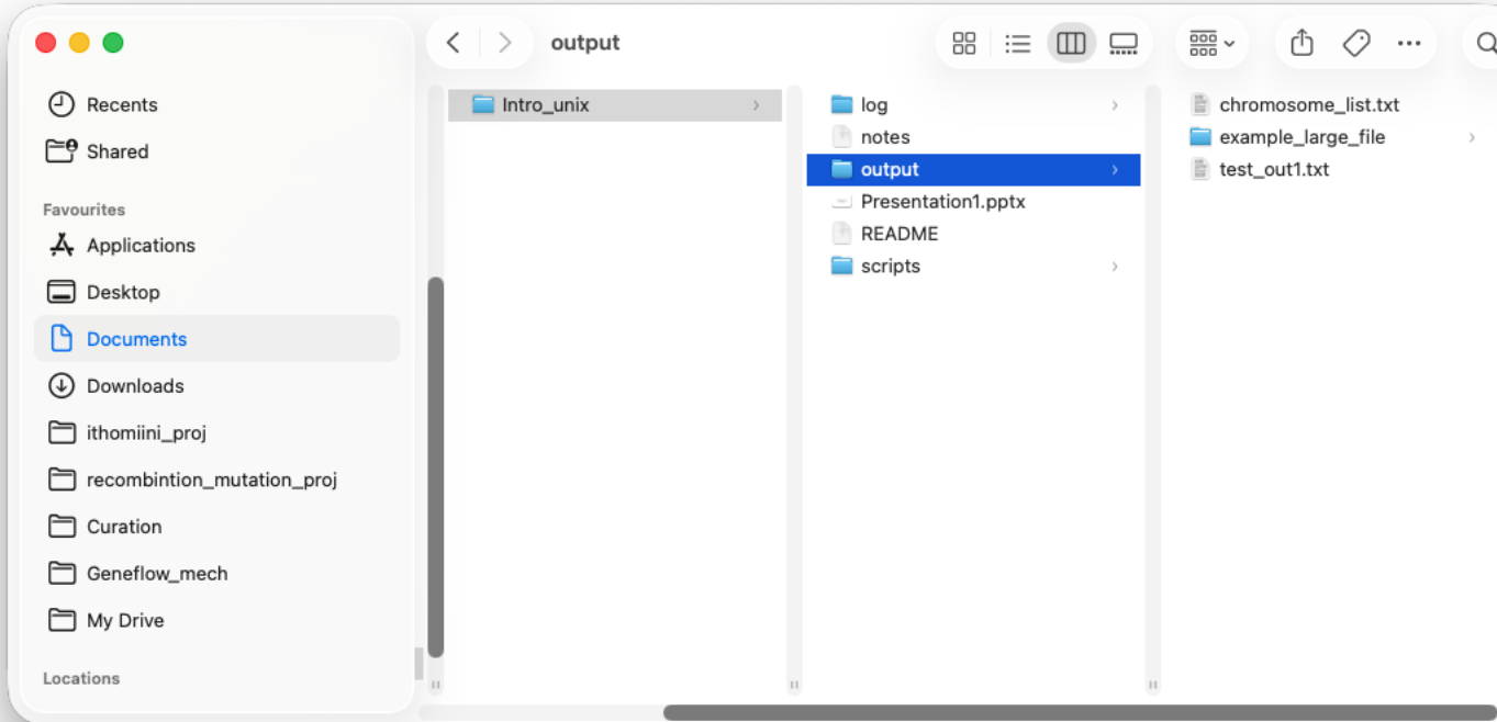
GUI (Finder)
