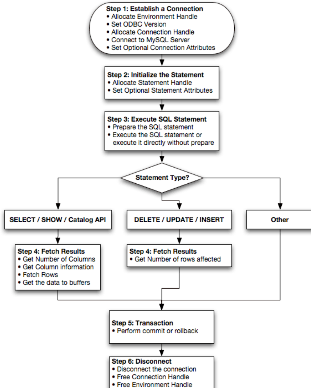
Figure 6.1 Connector/ODBC Programming Flowchart
