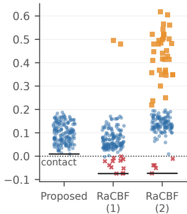
(c) Clearance to obstacles
