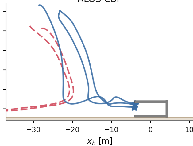
ALOS CBF
