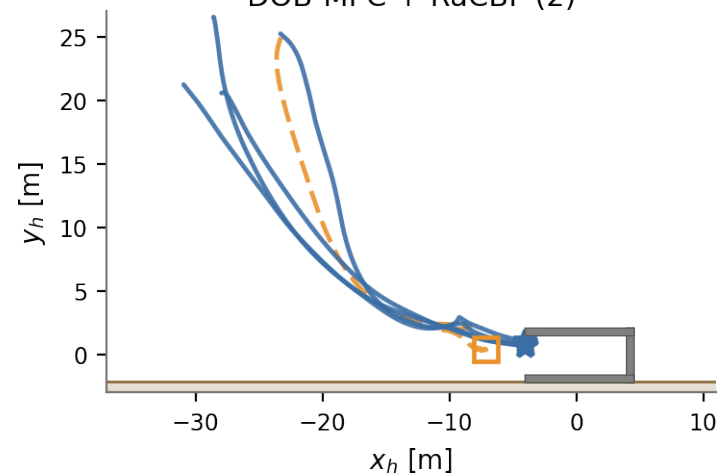
DOB-MPC + RaCBF (2)
