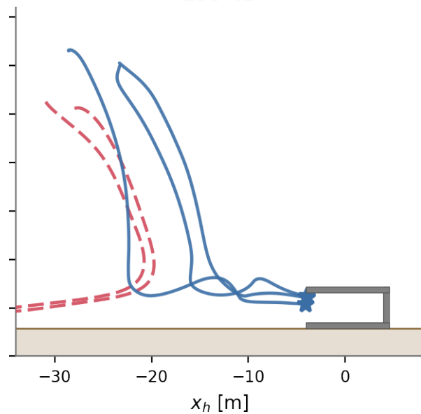
ALOS CBF
