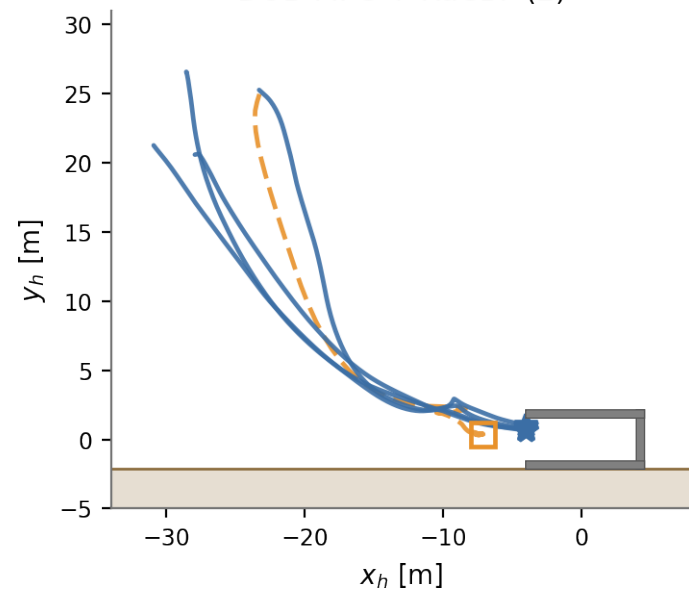
DOB-MPC + RaCBF (2)
