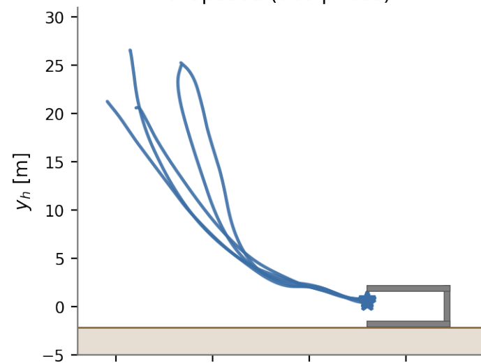
DOB-MPC + RaCBF (2)
