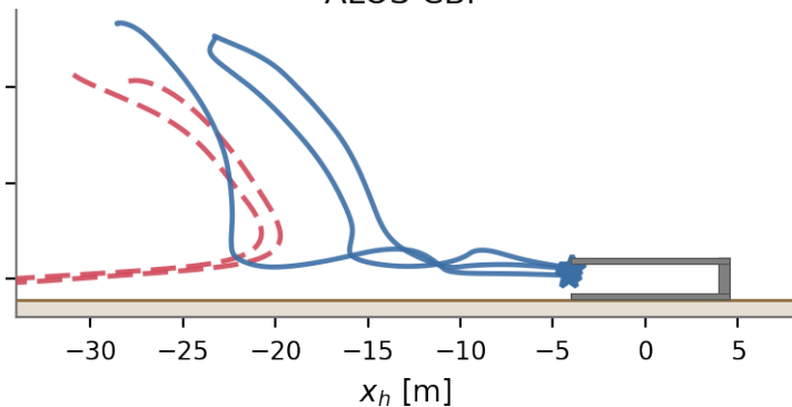
ALOS CBF
