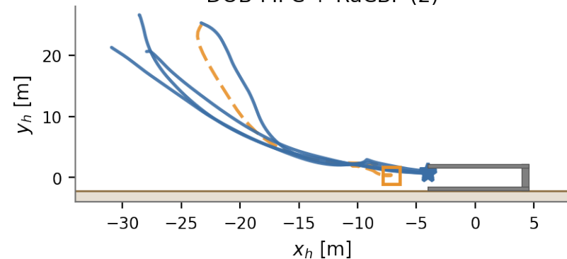
DOB-MPC + RaCBF (2)
