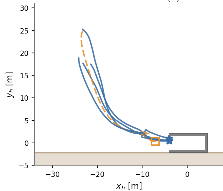
DOB-MPC + RaCBF (2)
