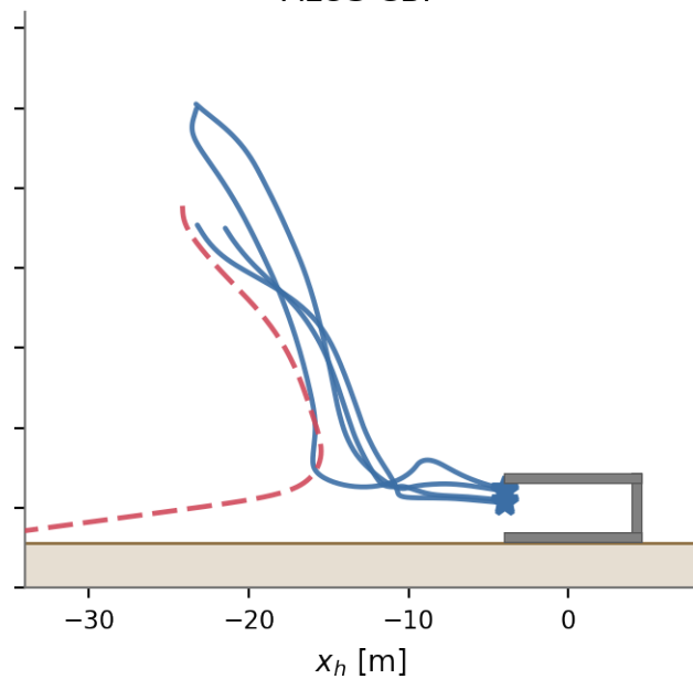
ALOS CBF
