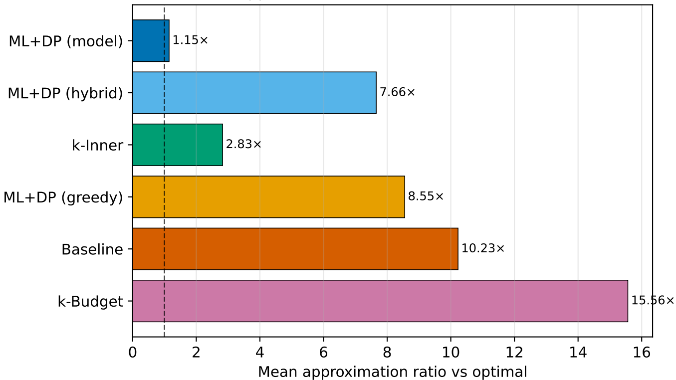
Overall approximation ratio (held-out test set, n=200)
