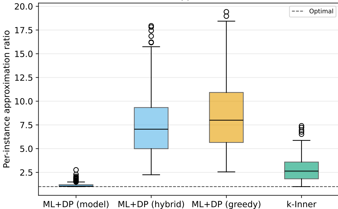
Distribution of approximation ratios
