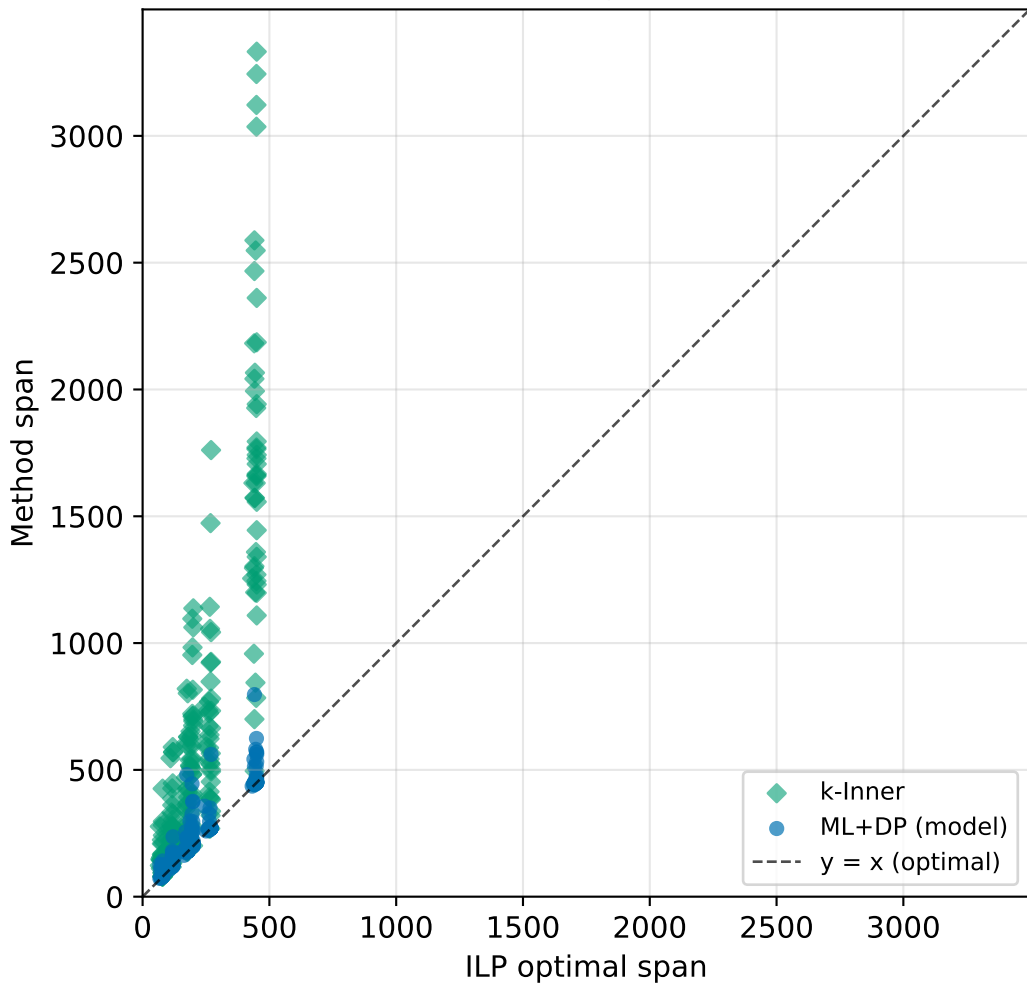
Per-instance span vs optimum (closer to the diagonal is better)
