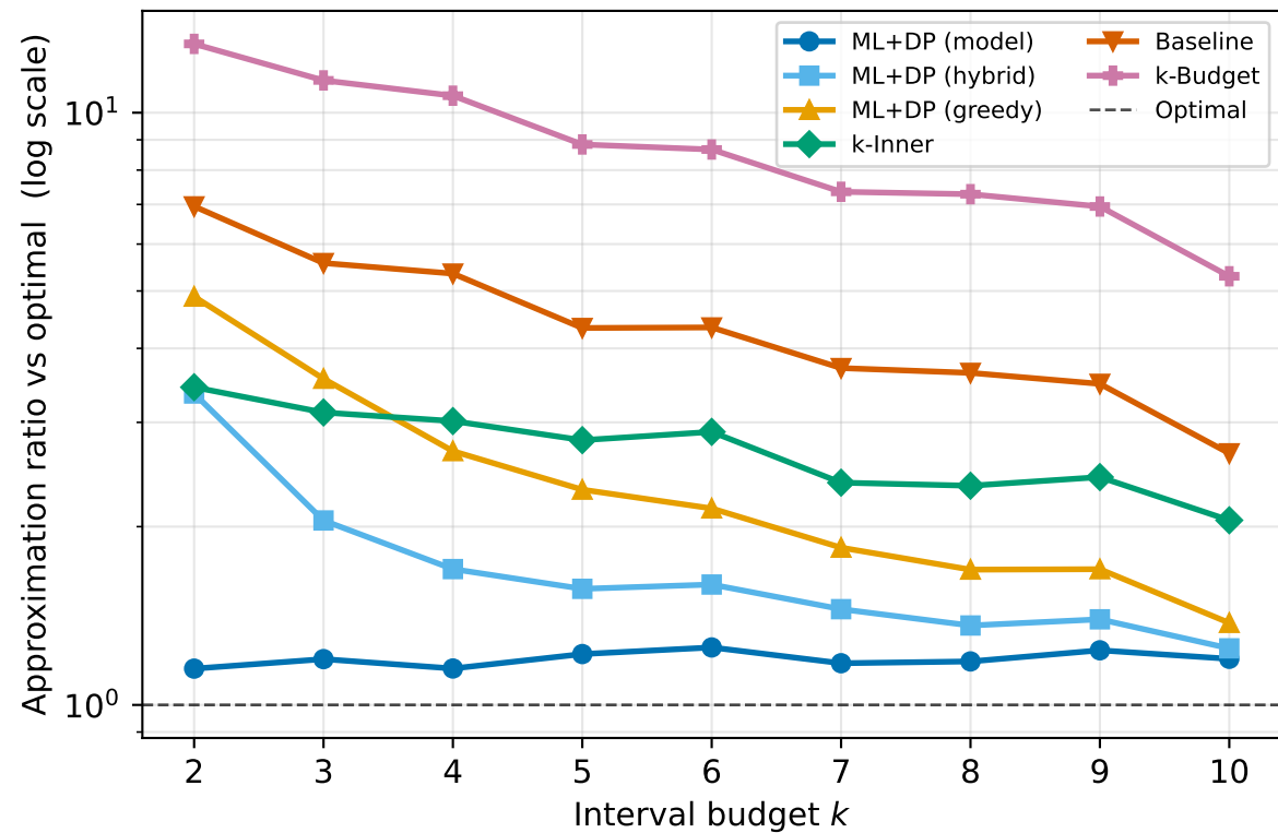
Approximation ratio by k (lower is better)
