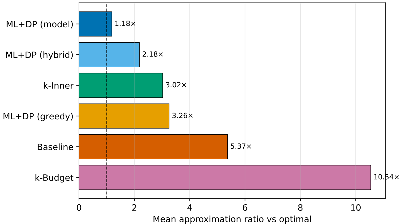
Overall approximation ratio (held-out test set, n=200)
