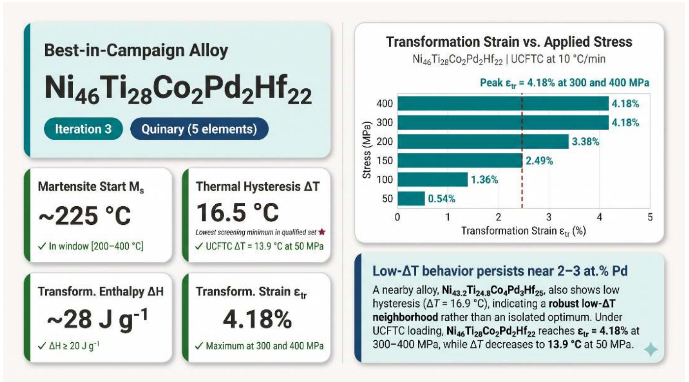
Figure 5: Summary of the highest-performing alloy identified during the Bayesian optimization campaign, Ni 46 Ti 28 Co 2 Pd 2 Hf 22 (Iteration 3). The alloy satisfies all four performance benchmarks and exhibits the lowest thermal hysteresis ( \Delta T = 16.5 °C) and highest measured transformation strain ( \epsilon_{tr} = 4.18\% ) among the fully qualified compositions. Property panels summarize the key screening metrics, including martensite start temperature ( M_s ), thermal hysteresis ( \Delta T ), transformation enthalpy ( \Delta H ), and transformation strain ( \epsilon_{tr} ). The bar chart shows the evolution of \epsilon_{tr} with applied stress during uniaxial constant-force thermal cycling (UCFTC). The figure also highlights the persistence of low-hysteresis behavior in nearby Pd-containing compositions and the reduction of \Delta T under applied load. Figure generated using Gemini and subsequently reviewed and edited by the authors.
