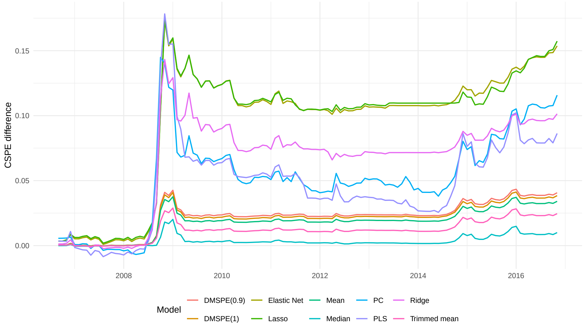
Cumulative forecast performance relative to historical average
