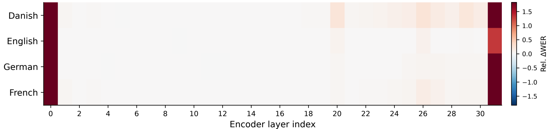
Layer importance ( \Delta WER when layer removed)
