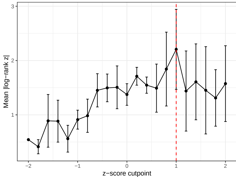
Mean |\log\text{-rank } z| by cutpoint
