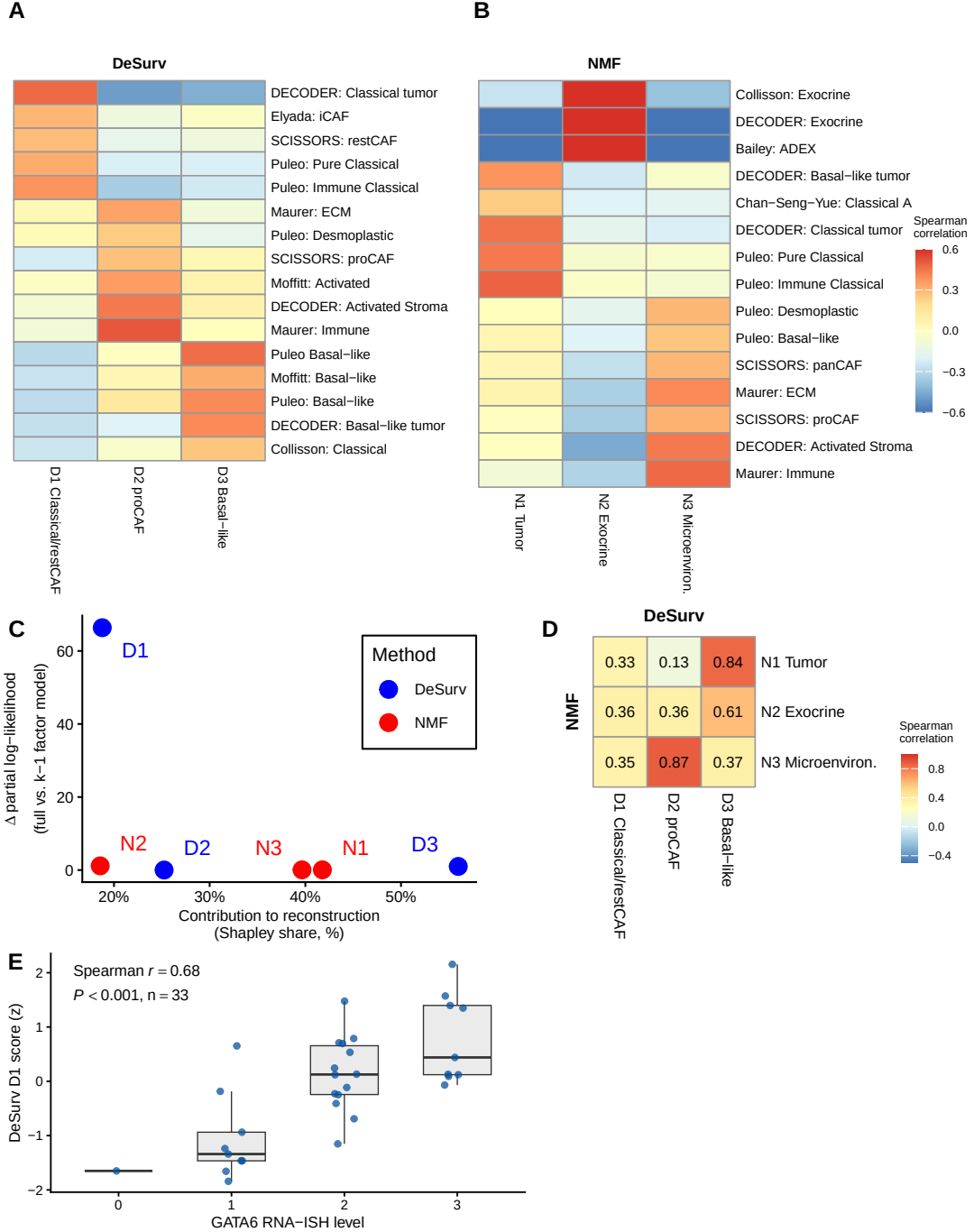
Figure 2: Survival supervision produces different factor structures in PDAC (TCGA + CPTAC training cohort, n = 273 patients, 139 events). (A,B) Spearman correlations between factor gene rankings (top 50 genes per factor) and established PDAC gene programs for DeSurv (A) and standard NMF (B) at k = 3 ; only |r| > 0.2 shown. (C) Per-factor reconstruction contribution (normalized Shapley share, summing to 100%) versus survival contribution ( \Delta Cox partial log-likelihood on factor removal). (D) Pairwise correspondence between NMF and DeSurv factors (Spearman correlation of W-matrix gene loadings over all genes). (E) DeSurv D1 score versus GATA6 RNA in situ hybridization level in the COMPASS cohort (Spearman correlation; n = 33 ).
