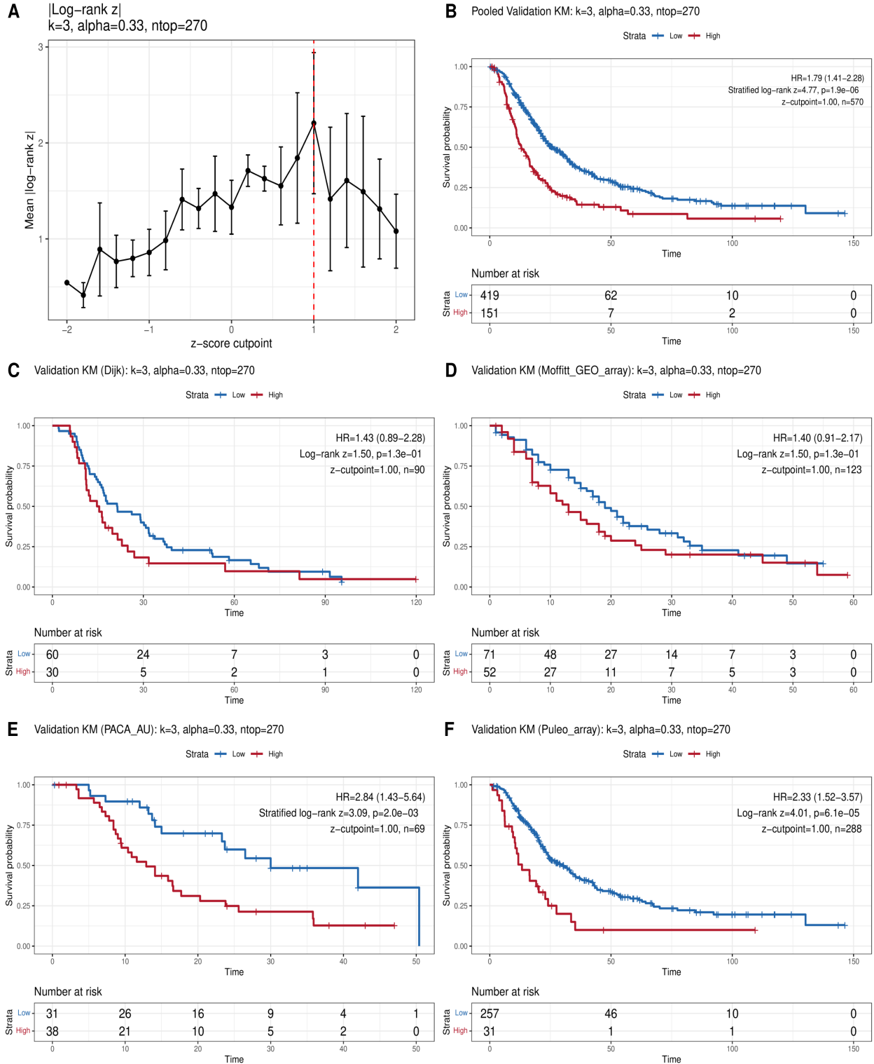
Figure S5: Cutpoint selection and external validation of dichotomized risk groups. (A) Cross-validated mean absolute log-rank z-statistic as a function of z-score cutpoint; red dashed line indicates the selected optimum. (B) Pooled validation Kaplan–Meier curves (stratified log-rank test). (C–D) Per-cohort validation KM curves: (C) Dijk, (D) Moffitt. (E–F) Per-cohort validation KM curves: (E) PACA-AU, (F) Puleo.
