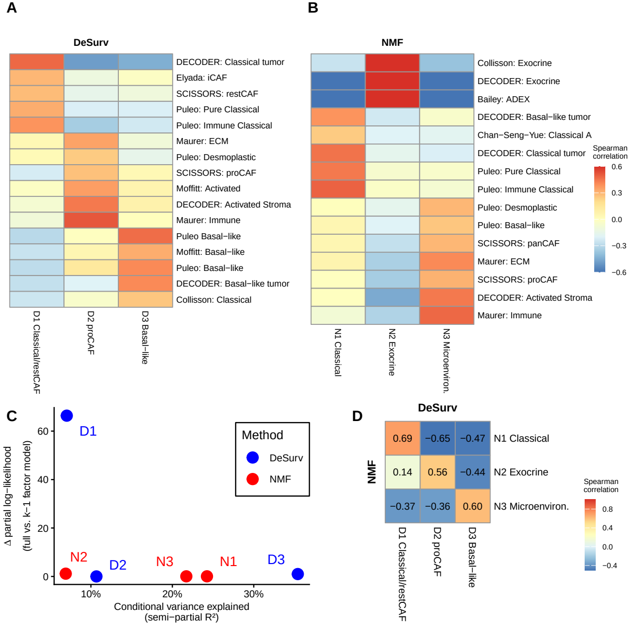
Figure 3: Survival supervision produces different factor structures in PDAC (TCGA + CPTAC training cohort, n = 273 patients, 139 events). (A–B) Spearman correlations between factor gene rankings (top 50 genes per factor) and established PDAC gene programs for DeSurv (A) and standard NMF (B) at k = 3 . Only |r| > 0.2 shown. DeSurv concentrates survival signal into D1 (Classical tumor + restCAF stroma) while suppressing exocrine variation; standard NMF devotes one factor to exocrine signals. (C) Fraction of expression variance explained versus survival contribution ( \Delta Cox partial log-likelihood upon factor removal) for each factor. DeSurv concentrates survival signal into D1 while the highest-variance NMF factor (N2, exocrine-associated) contributes negligibly to survival. (D) Pairwise correspondence between NMF and DeSurv factors, measured by Spearman rank correlation of W-matrix gene loadings restricted to the top 50 genes per factor.
