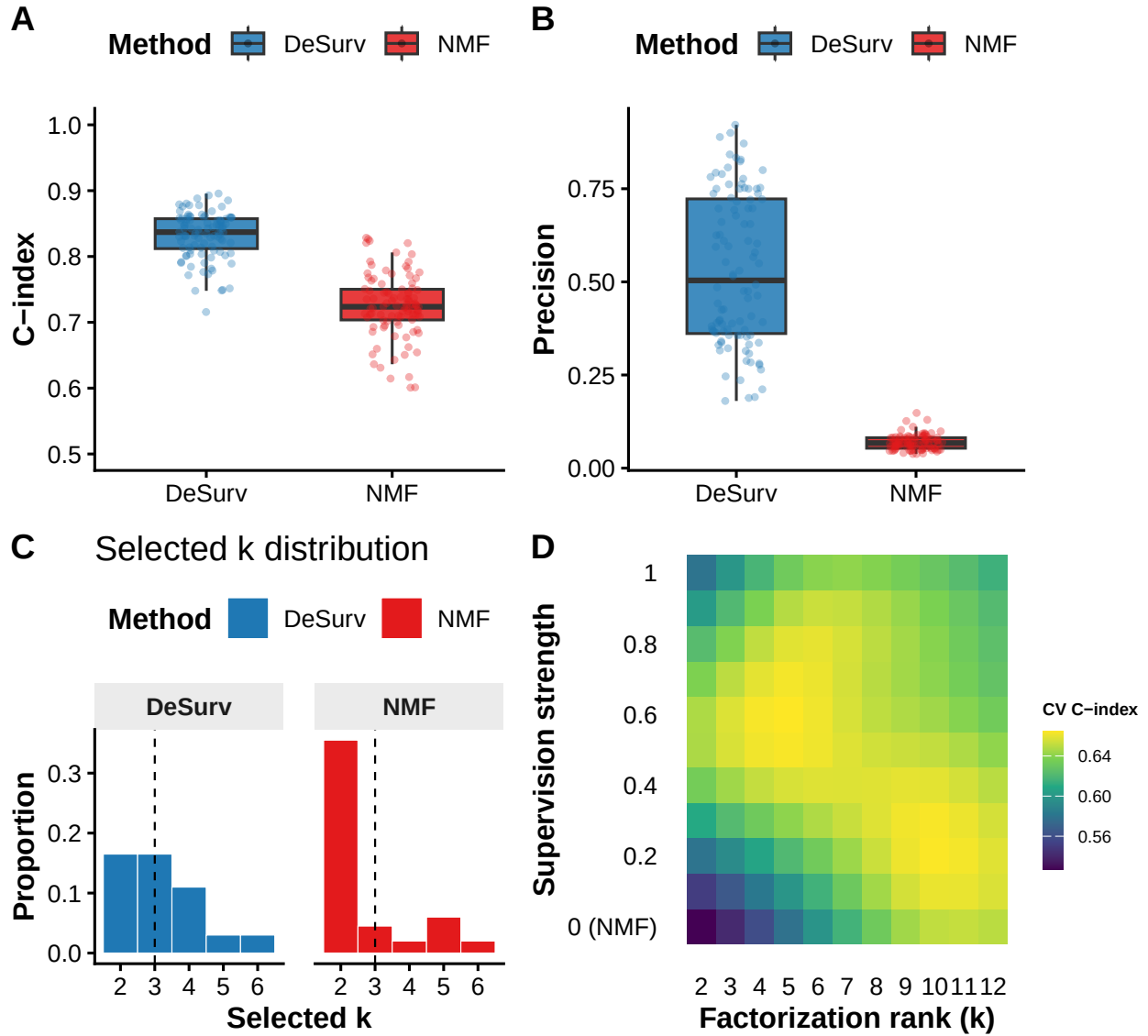
Figure 2: Simulation studies and model selection. (A) Test-set concordance index across 100 simulation replicates ( p = 3,000 genes, n = 200 samples, true k = 3 ) comparing DeSurv to standard NMF ( \alpha = 0 ); paired Wilcoxon P < 0.001 . (B) Precision (fraction of a factor’s top-weighted genes, defined in main text, overlapping a true prognostic program) across replicates. In (A) and (B), boxes show median and interquartile range (IQR); whiskers extend to 1.5 \times \text{IQR} ; points beyond are individual replicates. The y-axis in (A) is truncated at 0.5 because C-index values below 0.5 indicate worse-than-random concordance. (C) Distribution of selected k values across the same 100 replicates for DeSurv versus standard NMF. (D) Gaussian-process-predicted mean cross-validated C-index from Bayesian optimization over factorization rank ( k ) and supervision strength ( \alpha ) in PDAC training data (TCGA + CPTAC).
