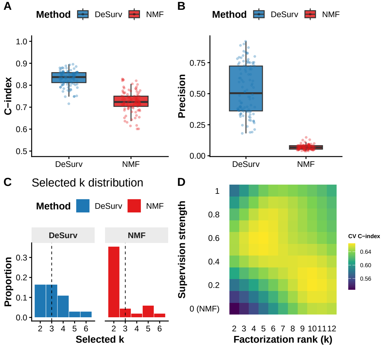
Figure 5: Survival supervision improves recovery of prognostic gene programs in simulations. (A) Test-set concordance across 100 simulation replicates comparing DeSurv with standard NMF ( \alpha = 0 ; p = 3,000 genes, n = 200 samples, true k = 3 ; paired Wilcoxon P < 0.001 ). (B) Precision of recovered prognostic gene programs (overlap between each true program and the top-weighted genes of its best-matching learned factor). In (A) and (B), boxes show median and interquartile range; whiskers extend to 1.5 \times \text{IQR} ; points are individual replicates. (C) Distribution of selected ranks across replicates for DeSurv versus standard NMF. (D) Gaussian-process-predicted mean cross-validated C-index over factorization rank and supervision strength in PDAC training data (TCGA + CPTAC); this panel shows empirical tuning, not a simulation result.
