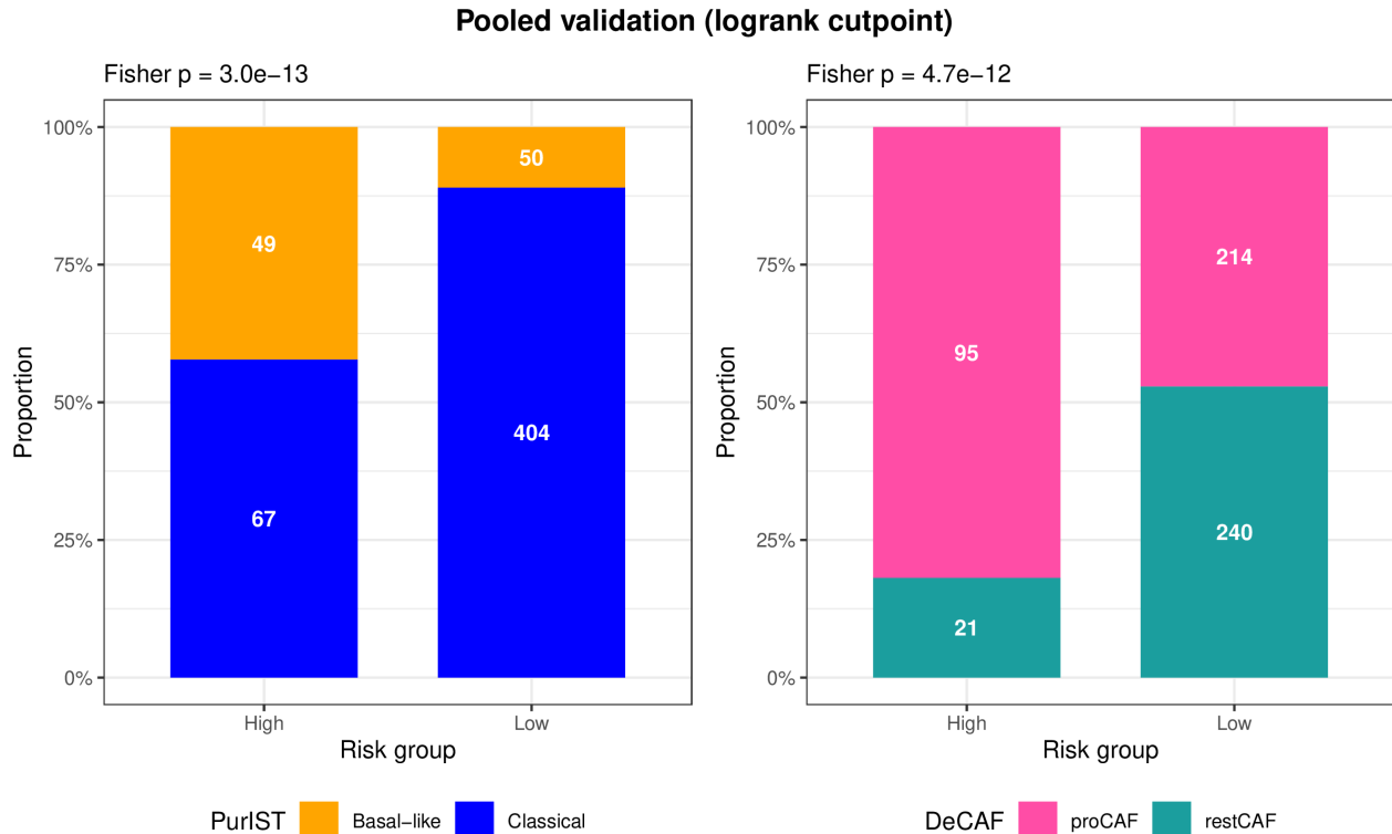
Figure S6: Subtype composition of DeSurv risk groups in pooled external validation cohorts. Stacked bar charts show the proportion of PurIST (left) and DeCAF (right) subtypes within Low and High risk groups defined by the log-rank-optimized cutpoint. Numbers indicate sample counts; Fisher's exact test P-values are shown above each panel.
