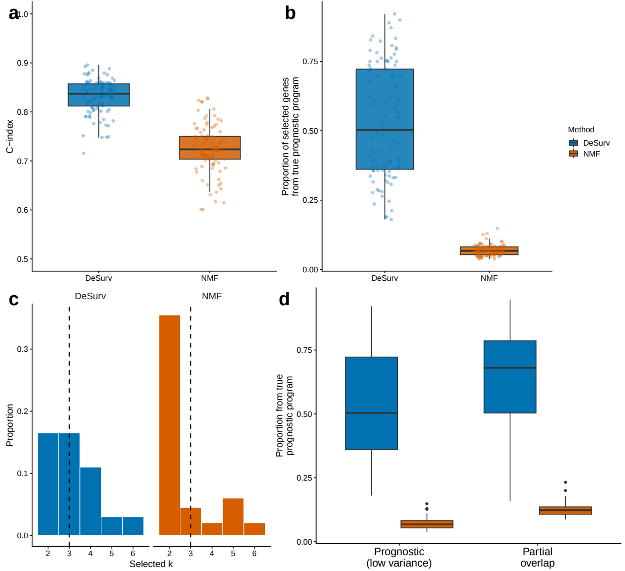
Figure 5: Survival supervision improves recovery of prognostic gene programs when prognostic signal contributes relatively little expression variation. (a) Test-set concordance across 100 simulated datasets comparing DeSurv with unsupervised NMF ( \alpha = 0 ; p = 3,000 genes, n = 200 samples, true k = 3 ); median C-indices were 0.837 versus 0.724 (paired Wilcoxon P < 0.001 ). (b) Recovery of genes defining the true prognostic program, quantified as the proportion of selected genes in the best-matching learned program that belonged to the ground-truth prognostic gene set; medians were 0.50 versus 0.07. The best-matching program is selected using the known simulated gene set, so this metric evaluates recovery with access to ground truth. Global marker recall, which requires no factor matching, is reported in the Supplementary Information. In (a) and (b), boxes show medians and interquartile ranges, whiskers extend to 1.5 \times \text{IQR} , and points represent individual simulated datasets. (c) Distribution of ranks selected across simulated datasets for DeSurv and unsupervised NMF; dashed lines indicate the true rank ( k = 3 ). (d) The same matched-factor precision metric as in (b) under two signal regimes: a prognostic program whose genes contribute relatively little transcriptomic variation and are separated from the dominant shared background, and a setting in which the survival-generating gene set partially overlaps that dominant background structure. DeSurv recovered the prognostic program more accurately in both regimes, with a larger separation when the prognostic program was distinct from the dominant expression structure. The null scenario, with no prognostic signal, is shown in the Supplementary Information. The concordance difference in (a) should not be interpreted as an expected gain in discrimination in real data, where a rank-optimized unsupervised control carried comparable prognostic information (Table 1).
