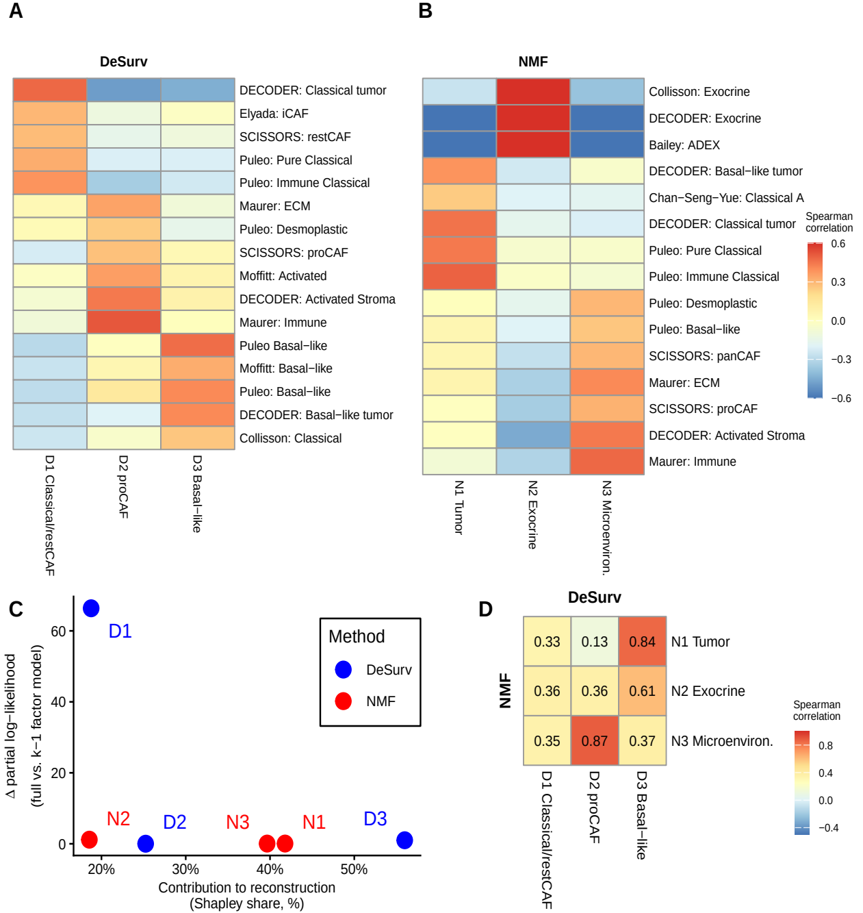
Figure 2: Survival supervision produces different factor structures in PDAC (TCGA + CPTAC training cohort, n = 273 patients, 139 events). (A–B) Spearman correlations between factor gene rankings (top 50 genes per factor) and established PDAC gene programs for DeSurv (A) and standard NMF (B) at k = 3 . Only |r| > 0.2 shown. DeSurv concentrates survival signal into D1, whose Classical-tumor + restCAF-like-stroma pole marks lower risk, while suppressing exocrine variation; standard NMF devotes one factor to exocrine signals. (C) Per-factor contribution to reconstruction of the expression matrix (normalized reconstruction Shapley share, which partitions and sums to 100%) versus survival contribution ( \Delta Cox partial log-likelihood upon factor removal). DeSurv concentrates survival signal into D1 while NMF’s largest-reconstruction factors — including the exocrine-associated factor N2 — contribute negligibly to survival. (D) Pairwise correspondence between NMF and DeSurv factors, measured by Spearman rank correlation of W -matrix gene loadings over all genes.
