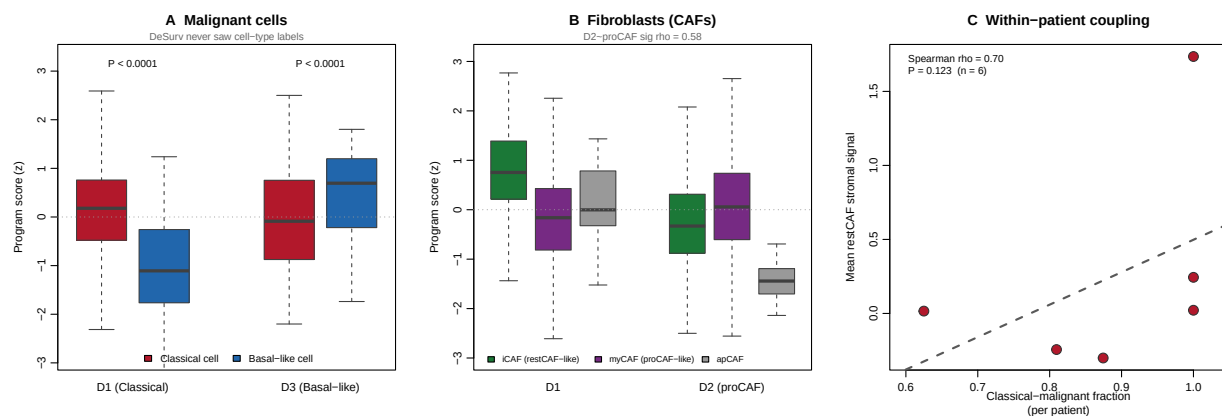
Figure 4: Frozen survival-supervised programs recover cell-resolved tumor and stromal states. The trained DeSurv program matrix was projected, without retraining and with no survival objective in play, onto an independent single-cell PDAC atlas using the same rank-and-project scoring as the bulk cohorts. (A) Mean program scores (D1, D2, D3) by cell state: D1 marks Classical malignant cells and restCAF-leaning fibroblasts, D3 marks Basal-like malignant cells, and D2 marks proCAF-leaning fibroblasts; the factorization was never given cell-type labels. (B) Within-patient co-occurrence: the per-patient fraction of Classical malignant cells versus mean restCAF stromal signal, the cellular-resolution form of the tumor–stroma coupling that defines D1.
