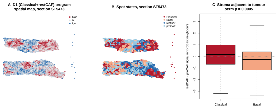
Figure 5: The tumor–stroma coupling is a reproducible spatial architecture. The frozen DeSurv programs were projected onto 7 independent Visium sections of human PDAC; spots were assigned to epithelial (Classical/Basal-like) or fibroblast (restCAF/proCAF) states from markers and the DeCAF stromal signatures. (A) Spatial map of the D1 (Classical+restCAF) program in a representative section, showing coherent tissue domains. (B) Spot-state map of the same section. (C) Stroma adjacent to tumour: in fibroblast spots neighbouring epithelium, the restCAF-minus-proCAF signal is positive next to Classical epithelium and negative next to Basal-like epithelium (within-section permutation test).
