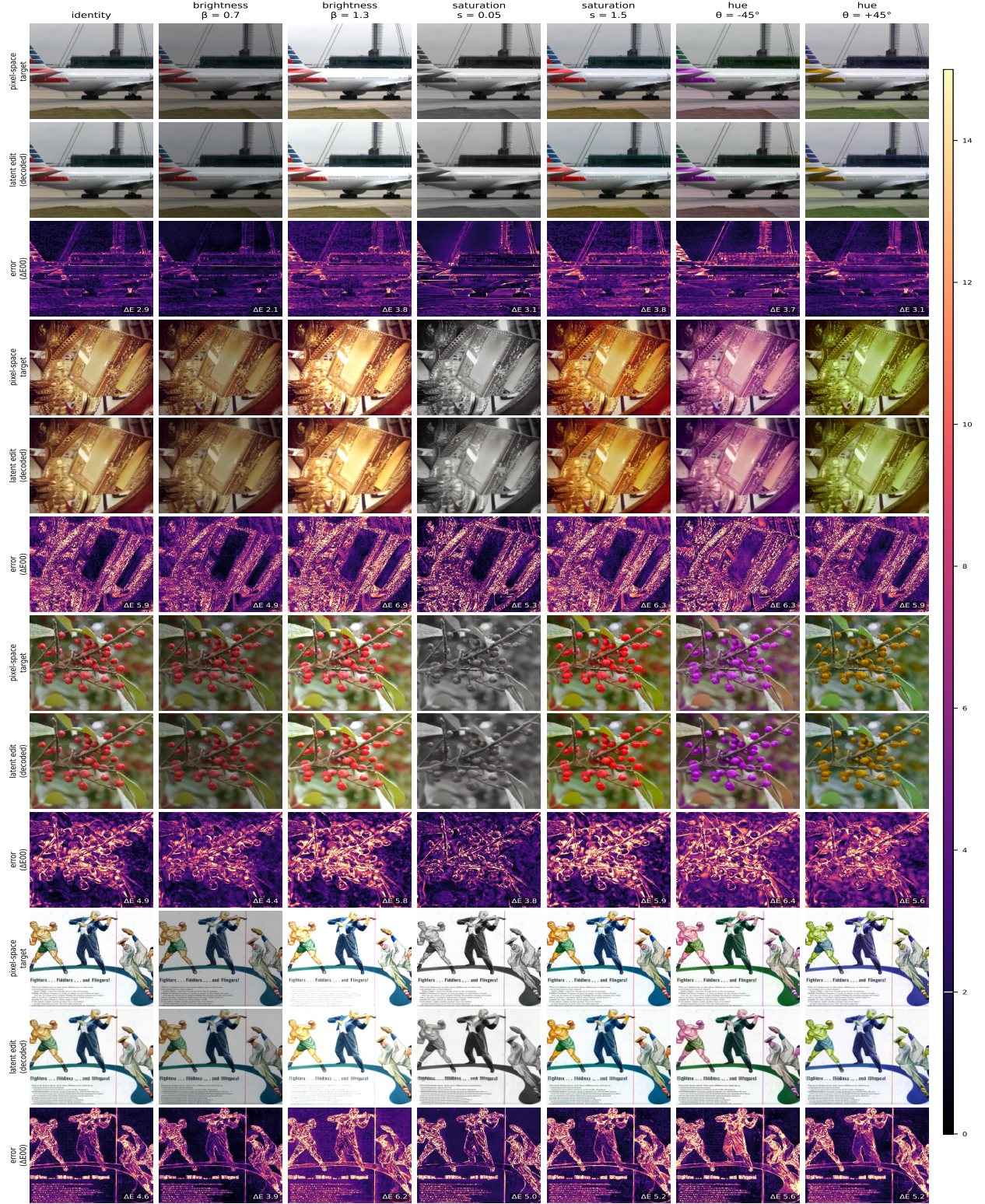
Figure 3: Latent-space color editing with the closed-form operator on the fine-tuned tokenizer. For each image: pixel-space targets \tau_a(x) (upper row), decoded latent edits D(T_a E(x)) (middle row), and the per-pixel \Delta E_{00} between them (lower row; shared 0–15 scale, colorbar tick at the \approx 2 JND), annotated with its mean. Each column applies Eq. (1) for the labeled transform directly to the latent before decoding. The identity column’s map is the reconstruction floor; the error concentrates on edges and fine texture rather than flat color regions, and the edit columns sit close to that floor and the operator-attributable error is the excess over the identity column.
