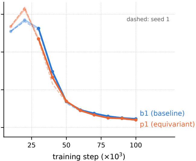
DiT-B/2 (130M), 2 seeds
