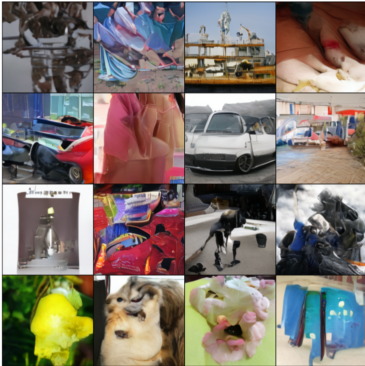
baseline (b1)
