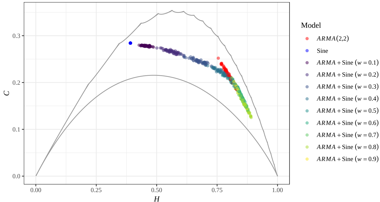
HC Plane — ARMA(2, 2) + \text{Sine} (50 reps, D = 4 )
