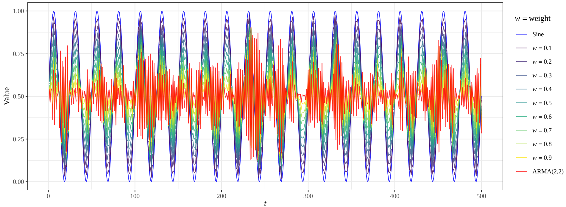
ARMA(2,2) + Sine convex combination
