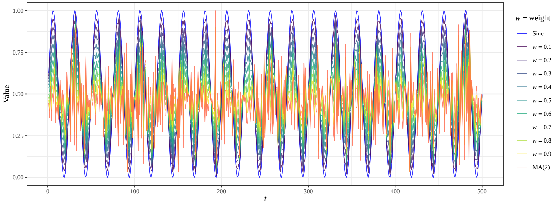
MA(2) + Sine convex combination
