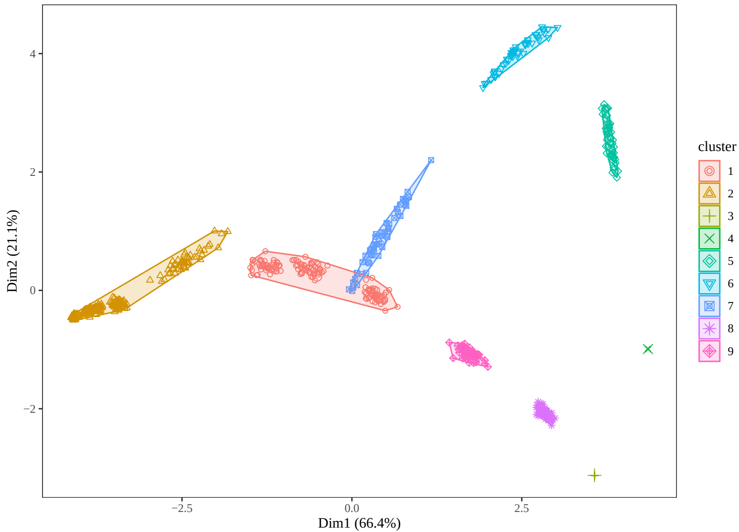
fviz_cluster | eps=0.8
