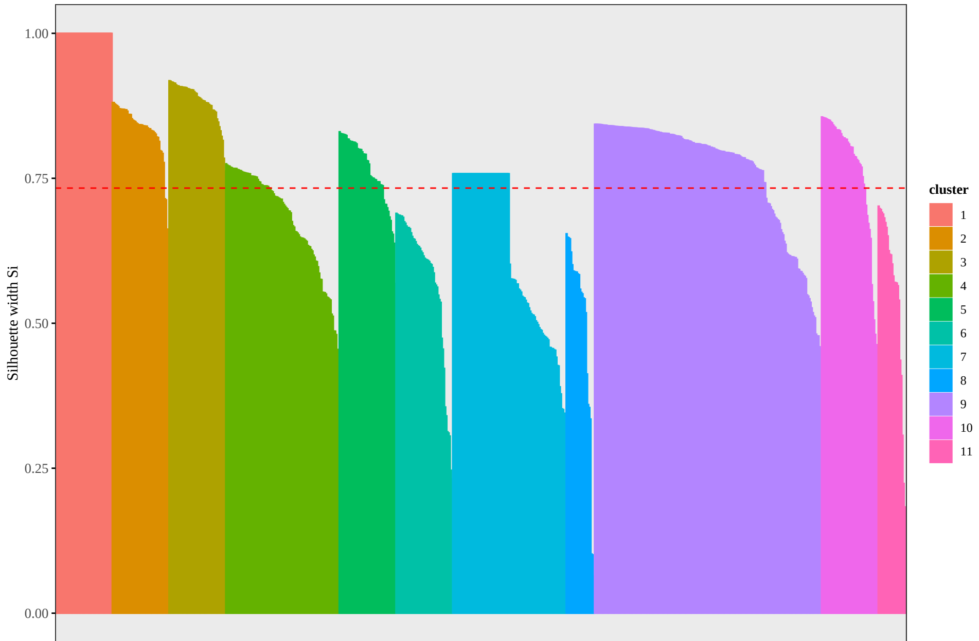
Silhouette Plot for k = 11
