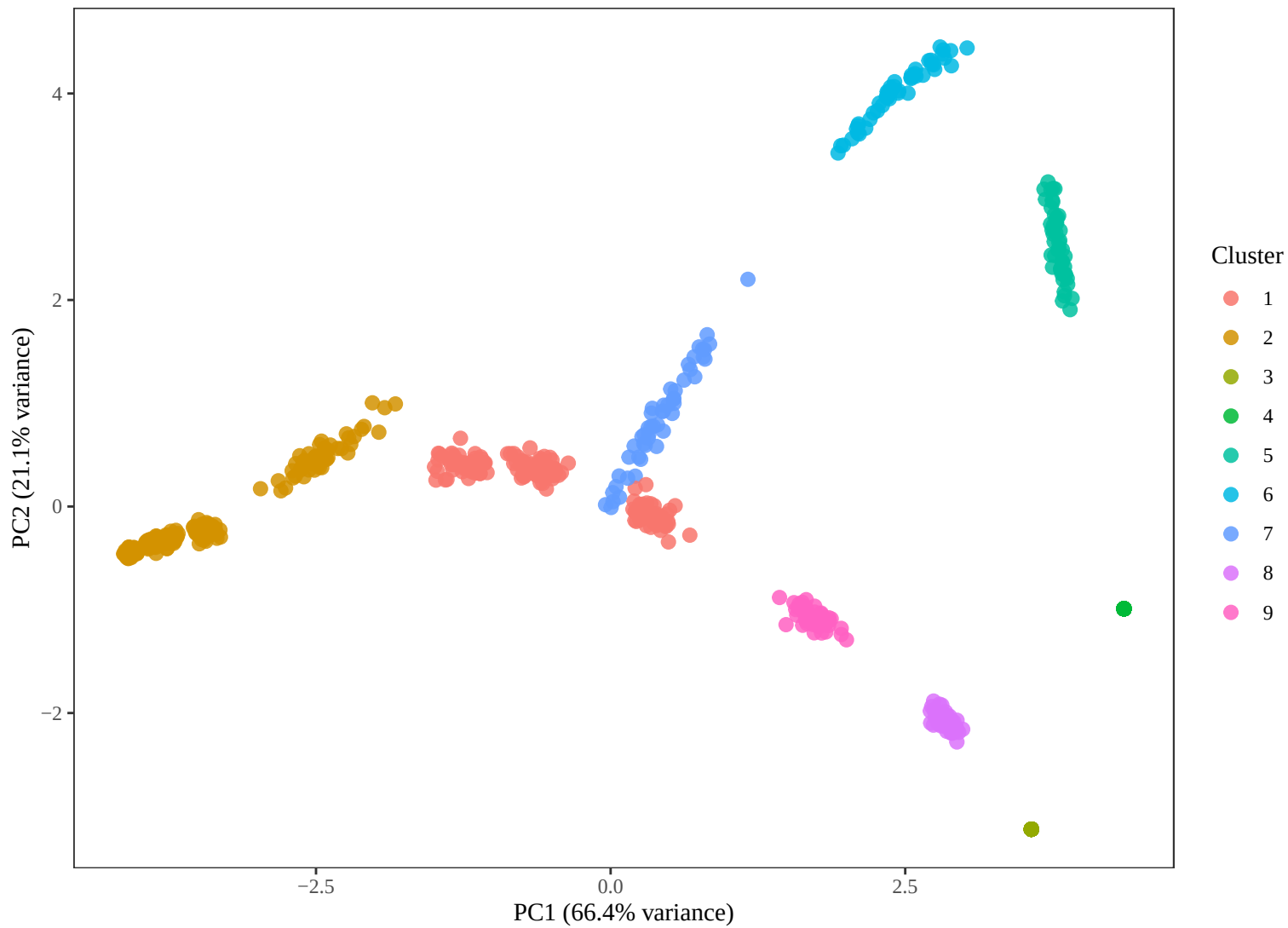
DBSCAN (eps=0.8, minPts=14)
