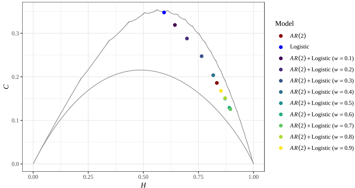
HC Plane — AR(2) + \text{Logistic } (D = 4)
