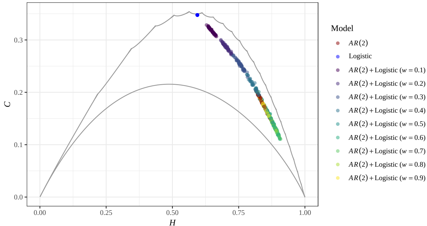
HC Plane — AR(2) + \text{Logistic} (50 reps, D = 4 )
