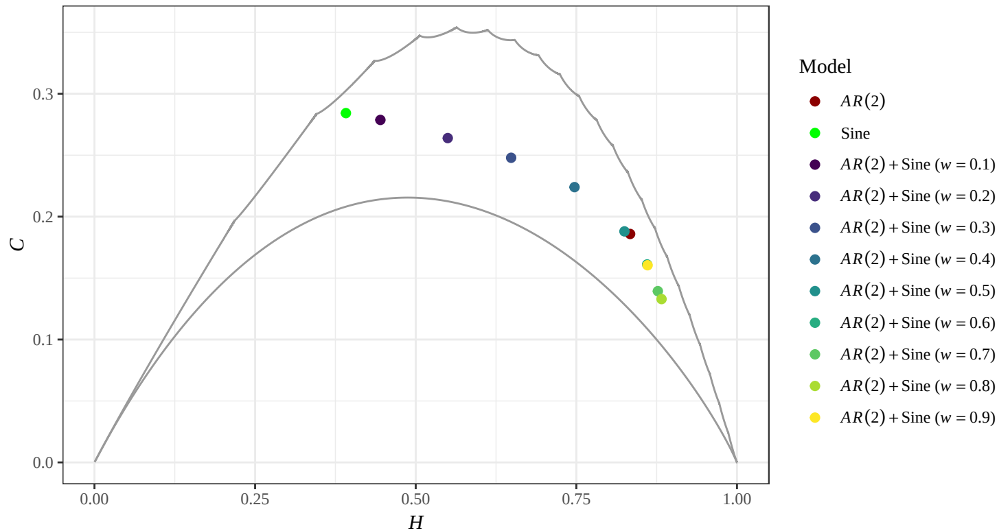
HC Plane — AR(2) + \text{Sine} ( D = 4 )
