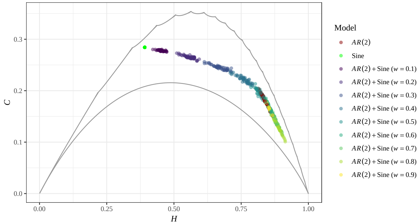
HC Plane — AR(2) + \text{Sine} (50 reps, D = 4 )
