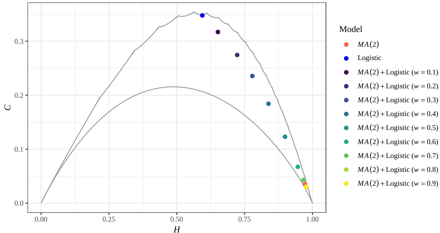
HC Plane — MA(2) + \text{Logistic } (D = 4)
