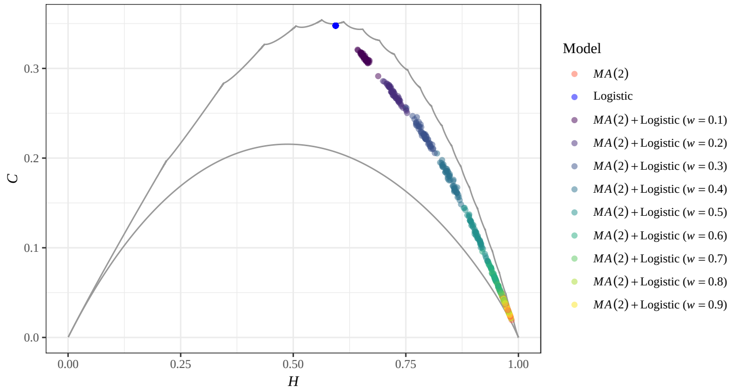
HC Plane — MA(2) + \text{Logistic} (50 reps, D = 4 )
